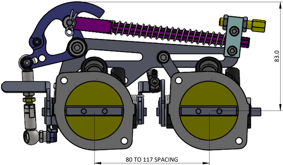
SINGLE LINKAGE SHOWN ON ST BODIES
