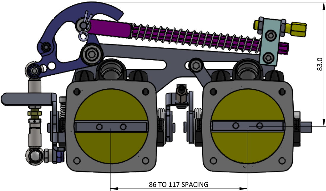
SINGLE LINKAGE SHOWN ON SF BODIES
